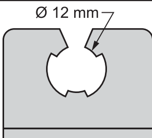
CN-12139 L= 38 mm H= 29 mm Endoscope holder, Ø 12 mm closed
