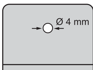
CN-12135 L= 38 mm H= 29 mm Endoscope holder, Ø 4 mm closed
