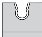
CN-12126 L= 23.5 mm H= 21 mm Ø 10.5 mm
