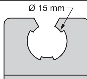
CN-12140 L= 38 mm H= 29 mm Endoscope holder, Ø 15 mm closed
