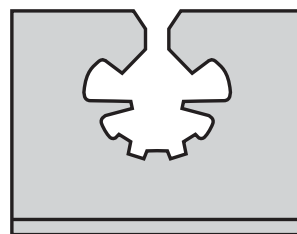
CN-12134 L= 38 mm H= 30 mm Endoscope holder, double one side 12 mm open one side from Ø 3 to Ø 8 mm
