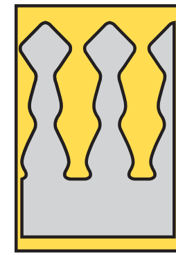
CN-12109 L= 238 mm H= 41 mm CN-12110 L= 158 mm H= 41 mm CN-12111 L= 112 mm H= 41 mm CN-12148 L= 77 mm H= 41 mm
